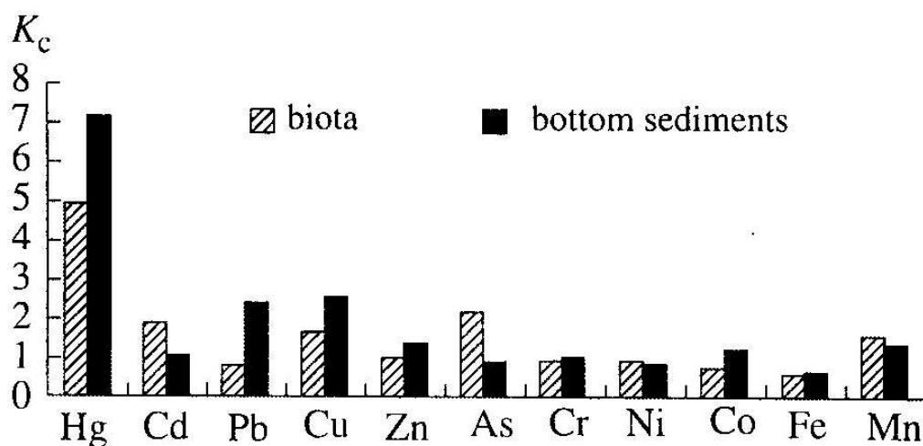
Fig. 4. Concentration coefficients K_c for mesoplankton ( A. salina ) and the upper layer of bottom sediments within the influence zone of the Ataihimprom chemical plant in Lake Bol'shoe Yarovoe (site 3).
