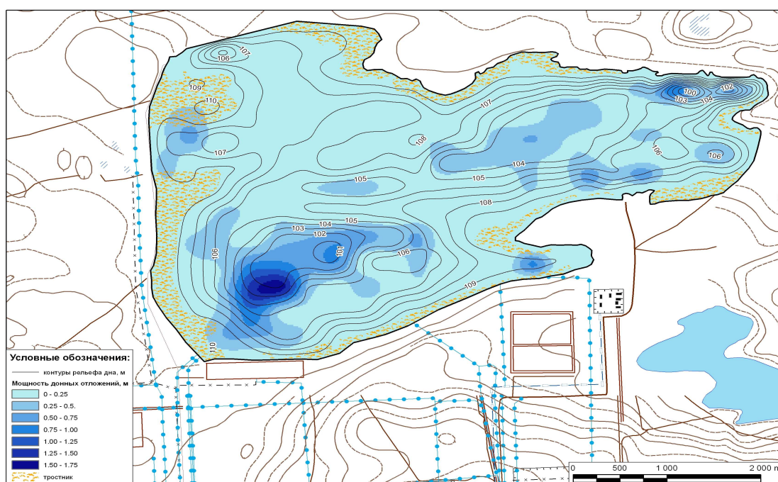
Figure 3. Wastewater storage pond Balkyldak bathymetric map and bottom sediments thickness
